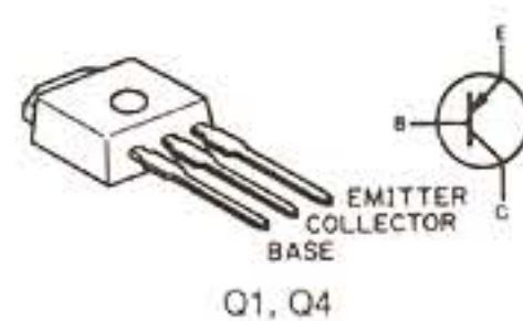
2SB1182
