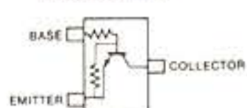
DTC144EU
