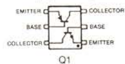
XP4312 (Symbol: 7T)
